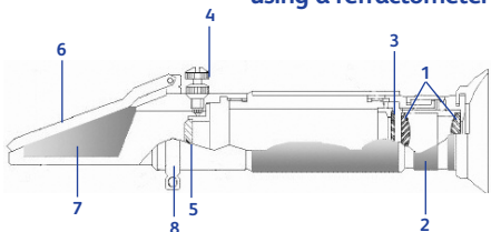
Figure 1. Refractometer schematic
